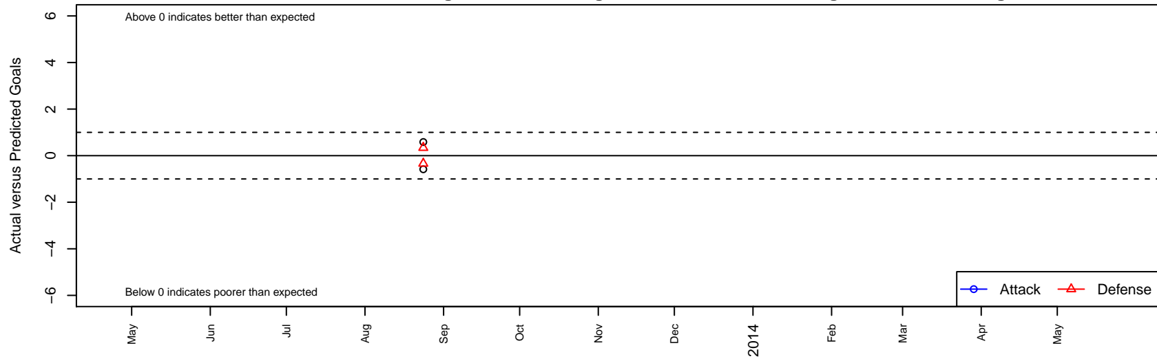
Fusion -Unk2 G00 Dots are actual minus expected GF (blue circles) and GA (red triangles). Blue line is smoothed change in attack strength. Red is smoothed change in defense strength.
